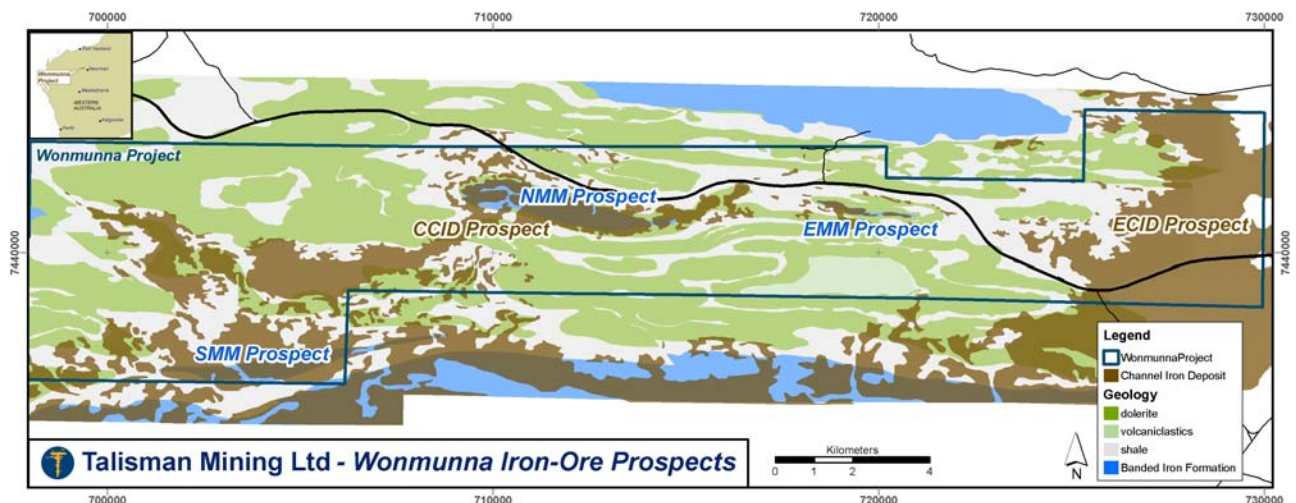
Figure 1: Wonmunna Project – Iron Prospects
